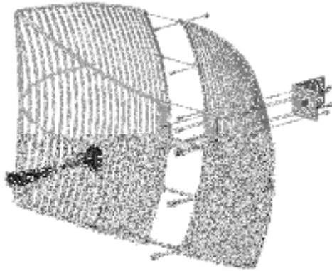
Figure 1: Illustration of Feed mounting to Grid Dish
